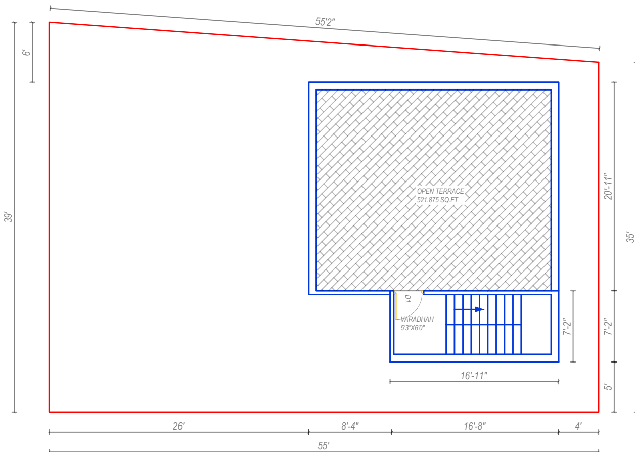
PROPOSED TERRACE FLOOR PLAN
